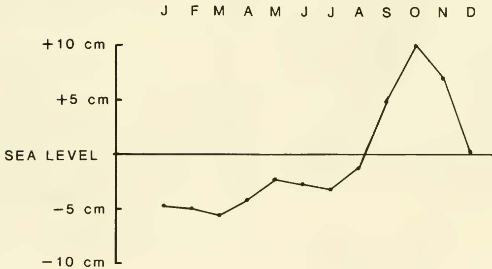
Figure 2. (a) A typical intertidal profile from south Florida showing the distribution of red and black mangrove (adapted from Provost 1974). (b) The pattern of annual sea level change in south Florida (Miami)(adapted from Provost 1974).
