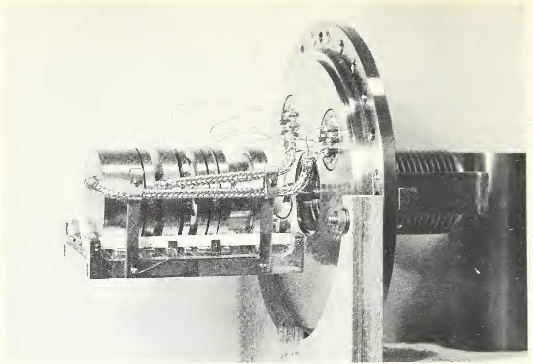
Inside of an electron optical bench which is used for testing electron optical components. It was set up at NBS to test a retarding field analyzer. (See p. 69.)
