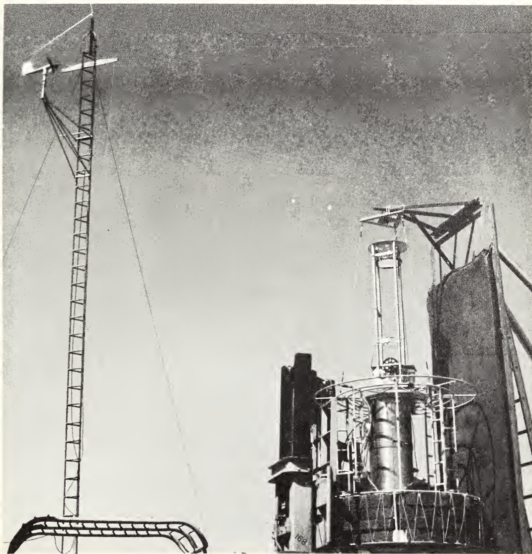
Balloon-borne spectrometer used to measure the composition of the atmosphere by means of its infrared absorption spectrum. The sun serves as the infrared source.
