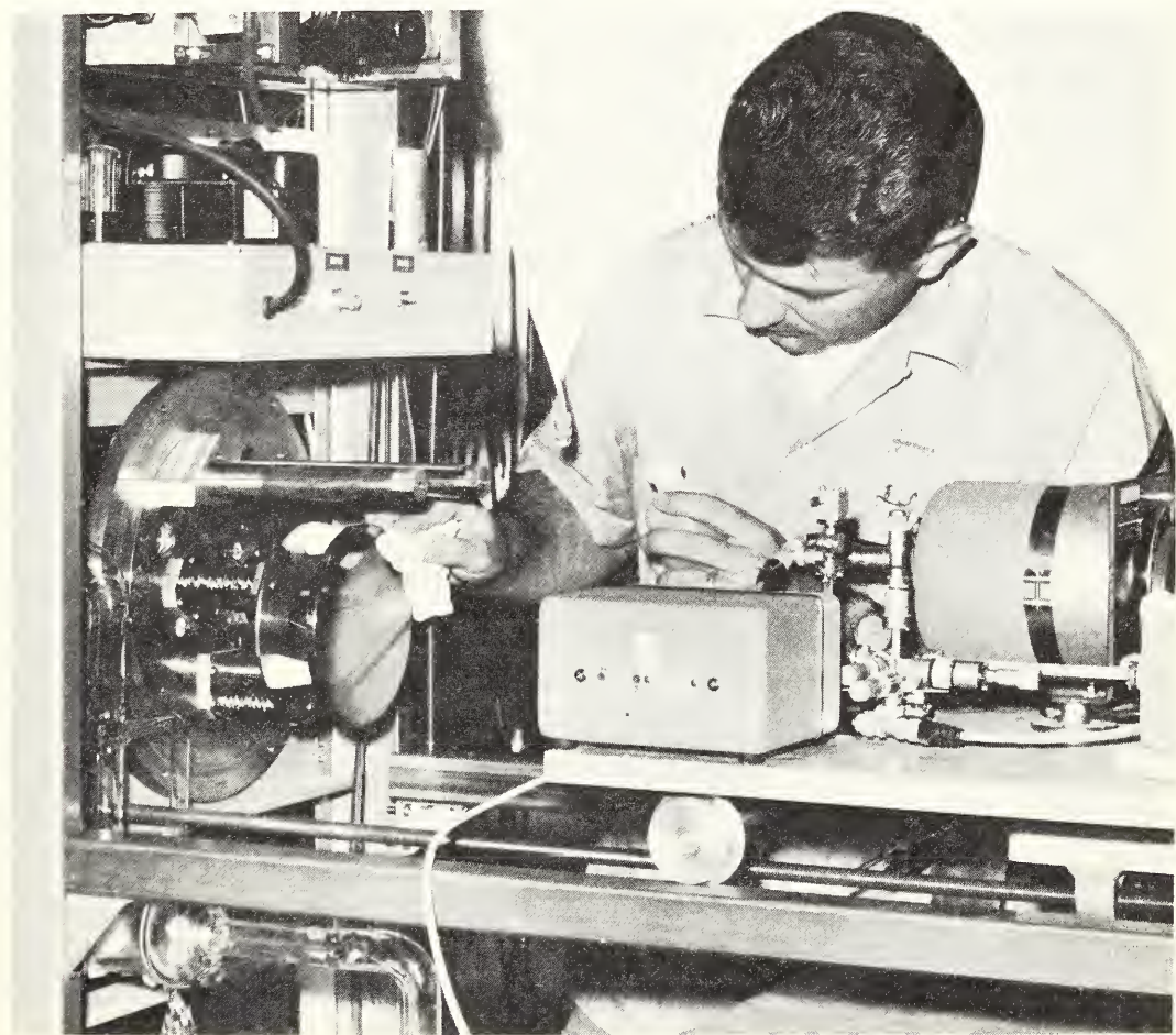
The Stark effect—splitting of spectral lines by the application of electric fields—is being investigated as a means for measuring d-c and low-frequency voltages to very high precision. This experiment employs millimeter wave techniques which were developed at NBS. (See p. 48.)
