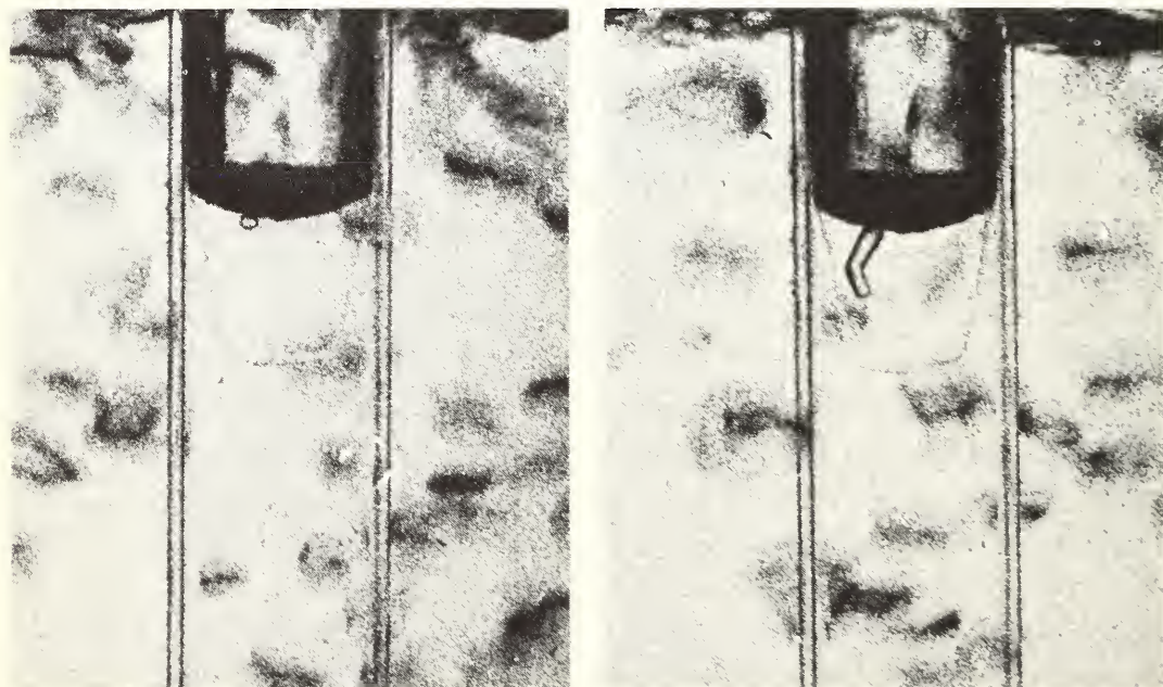
“Vapor snake” growing in crystallizing argon. Starting with a bubble at the surface of the melt (left) the snake grows downward as a vapor-filled solid sheath (right). This unusual phenomenon is shedding much light on the fundamental crystallization processes in the rare gases. (See p. 93.)
