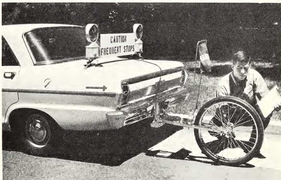
Checking the fifth wheel distance-measuring device used to obtain information regarding the accuracy of vehicle odometers. The investigation is designed to provide car-rental agencies with accuracy requirements, and to provide weights and measures officials with a performance code, testing equipment design, and test methods. (See p. 170.)
