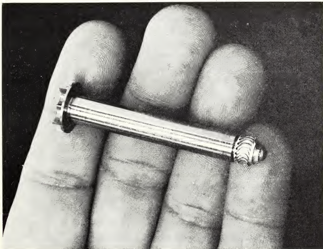
Miniature high-speed turbine expander is a vital component in a cryogenic refrigeration system. The turbine rotates at speeds up to 9000 revolutions per second. The shaft is supported by hydrostatic helium gas-lubricated bearings. (See p. 156.)
