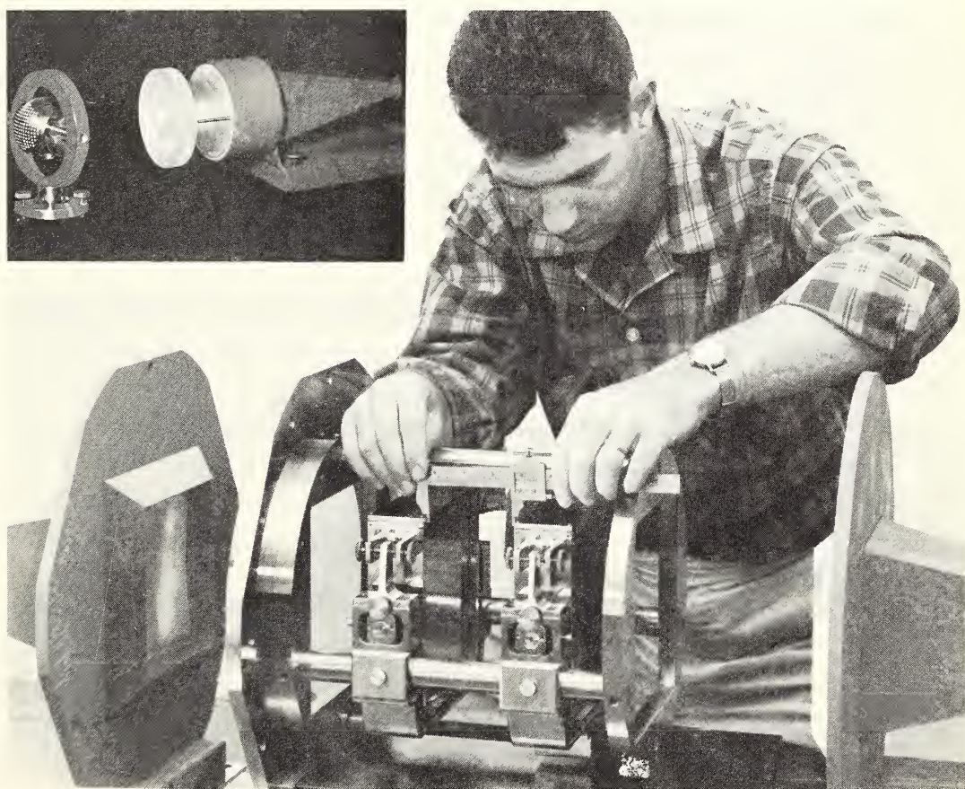
A Fabry-Perot Interferometer, designed to operate at millimeter wavelengths, is being used as the cavity resonator for a hydrogen cyanide gaseous maser. The device shows promise for frequency standard applications, and in microwave spectroscopy. Bi-conical, spherical cavity (inset) illustrates the design flexibility of the perforated cavities (page 44).
