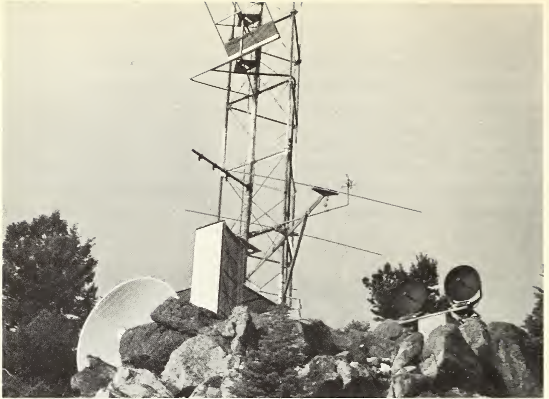
Mountain-top transmitting location for studies of fading characteristics in wide-band transmission systems. Receivers are located at a distance of 70 miles on the plains within the line-of-sight. Problems of space telecommunications have led to a need for more data on long line-of-sight transmission paths (page 128).
