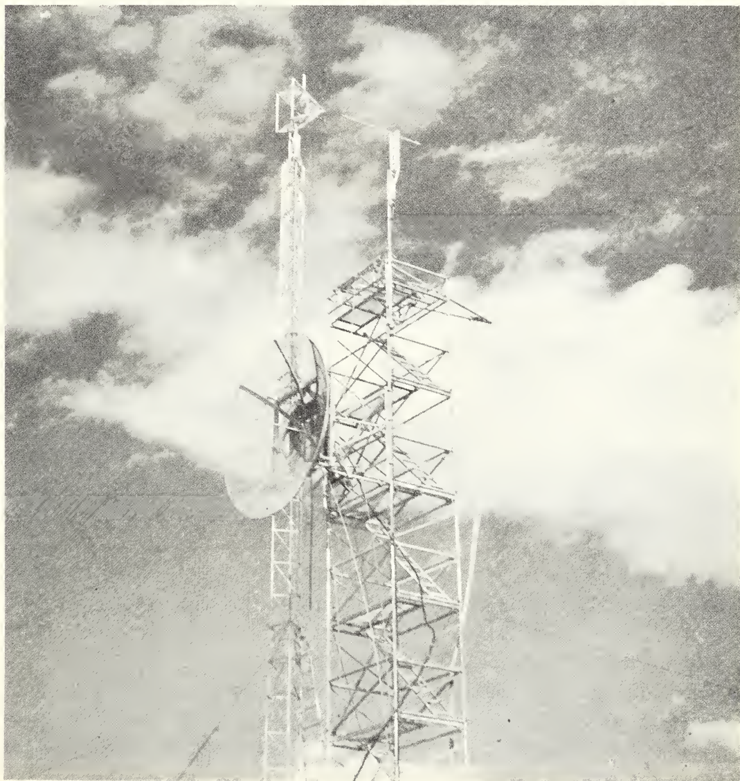
Receiving antennas used in studies of obstacle-gain propagation over Pikes Peak. Under certain conditions, signals propagated across mountain ridges are found to be far stronger than if the obstacle were not there (page 130).
