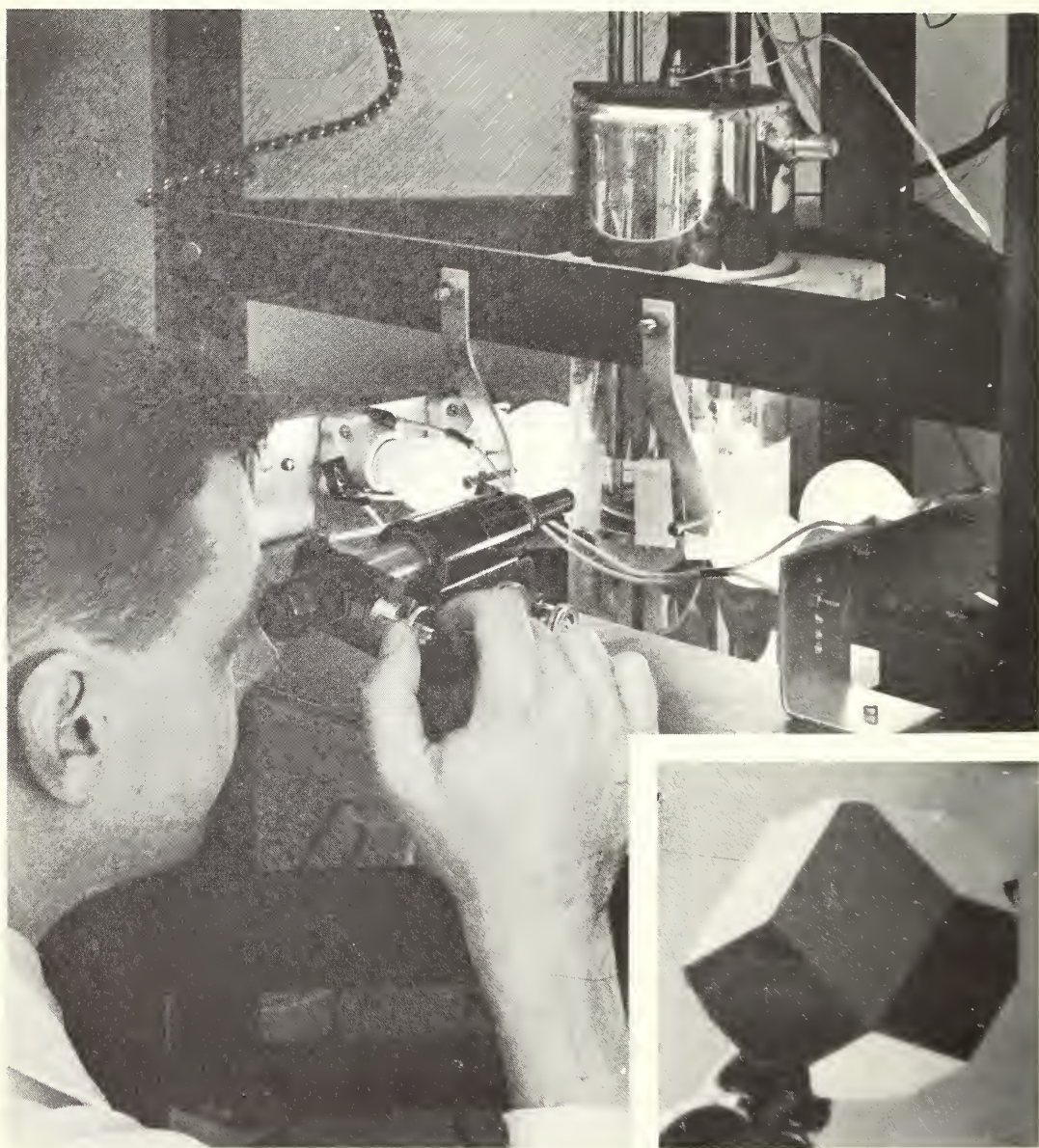
A measuring microscope is used to measure the distance between two faces on a potassium crystal growing from the vapor phase inside a dewar vessel. Inset shows potassium crystal about 0.9 mm in diameter. Studies of fundamental crystallization processes in metals provide a better understanding of the physical properties of the materials (page 92).
