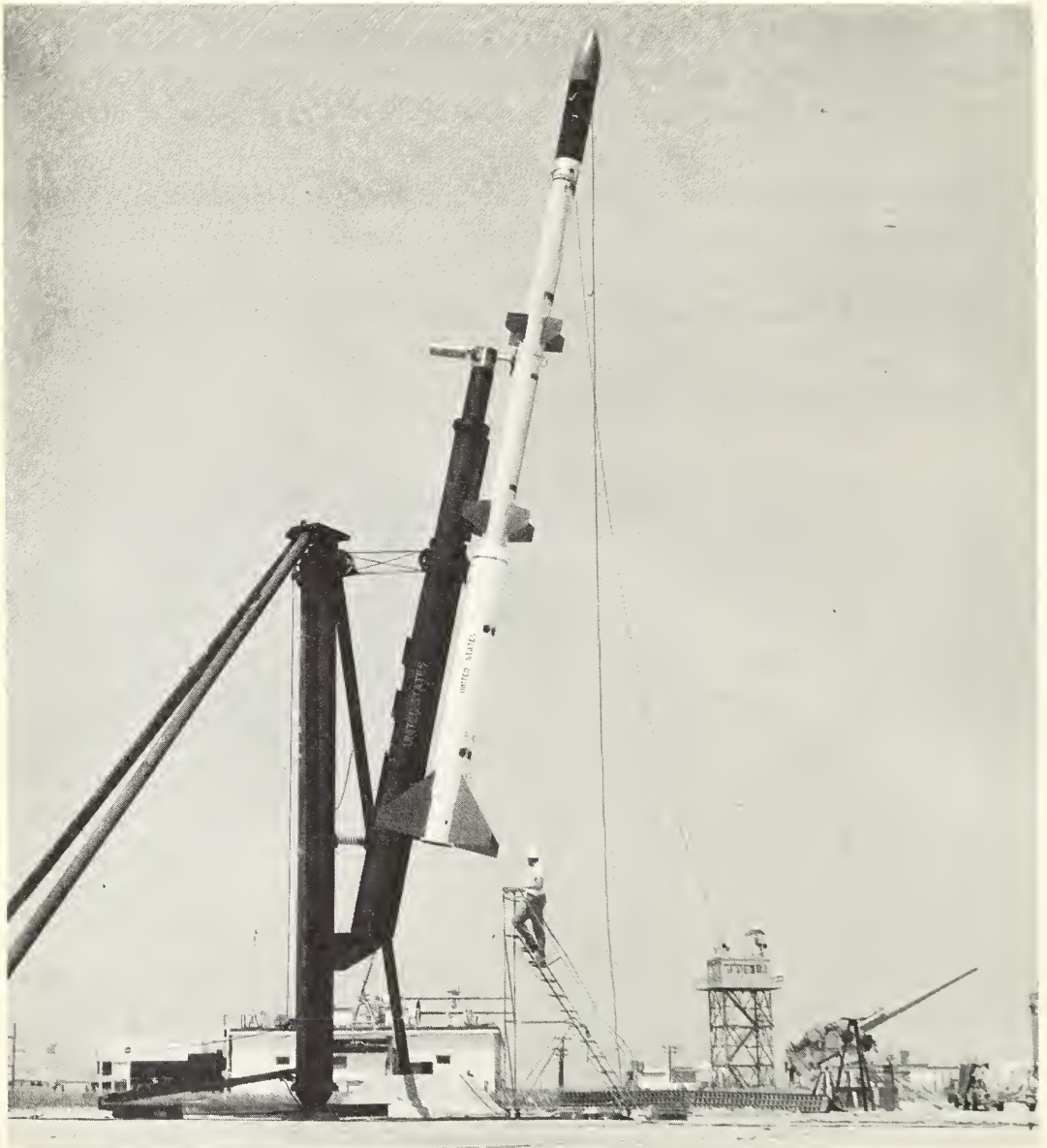
Javelin rocket which carried an ionosonde to an altitude of 1,000 kilometers. For thirteen minutes, the ionosonde made topside soundings of the ionosphere. The experiment was made to test the sounding system for the fixed-frequency satellite topside sounder to be orbited in 1962 (page 127).
