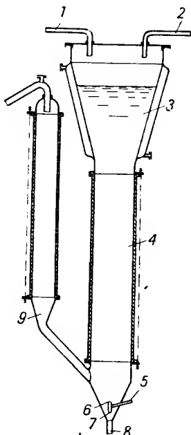
FIG. 50. Column for continuous manufacture of heavy metal azides and lead styphnate, according to Meissner [110]: 1,2— inflow of reacting solutions , 3,4— reaction column , 5— air nozzle with exit openings , 6 and 7 directed up- and downwards, respectively , 8— outlet , 9— overflow .
