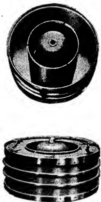
FIG. 198. Basket of a dehydration centrifuge, according to Brunswig [7].
