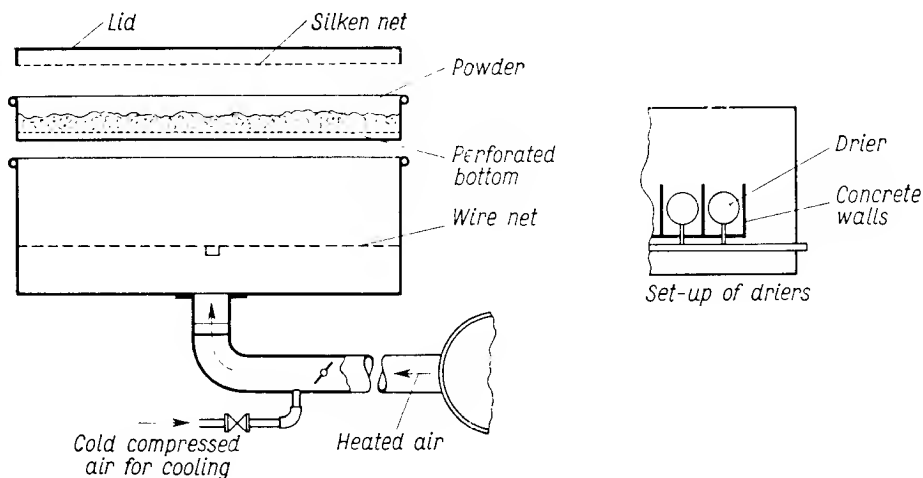
FIG. 239. Schematic view of a de Quinan drier.
