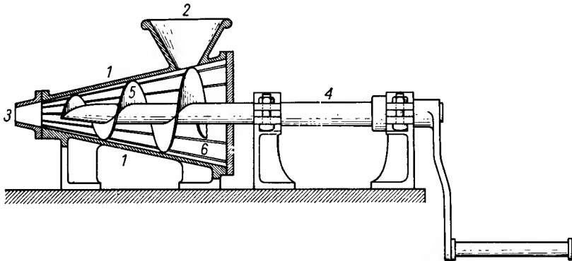
FIG. 178. Machine for the cartridgeing of dynamite [6].
