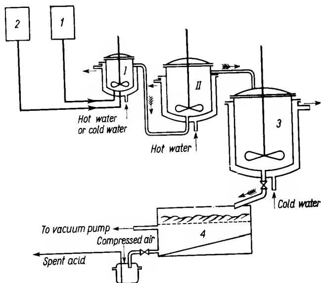
FIG. 8. Flow diagram of plant for continuous nitration of dimethylaniline.
