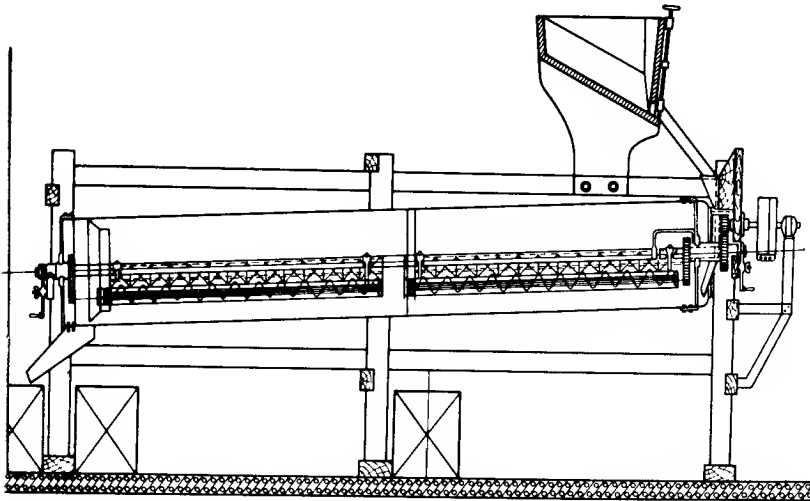
FIG. 234. Schematic view of a Marot installation for grading fine-grain powder (rotary screen), according to Yegorov [11].
