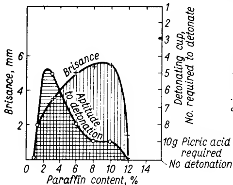
FIG. 72. Explosive properties of the mixtures of potassium chlorate with kerosene (according to Chemisch-Technische Reichsanstalt [73]).
