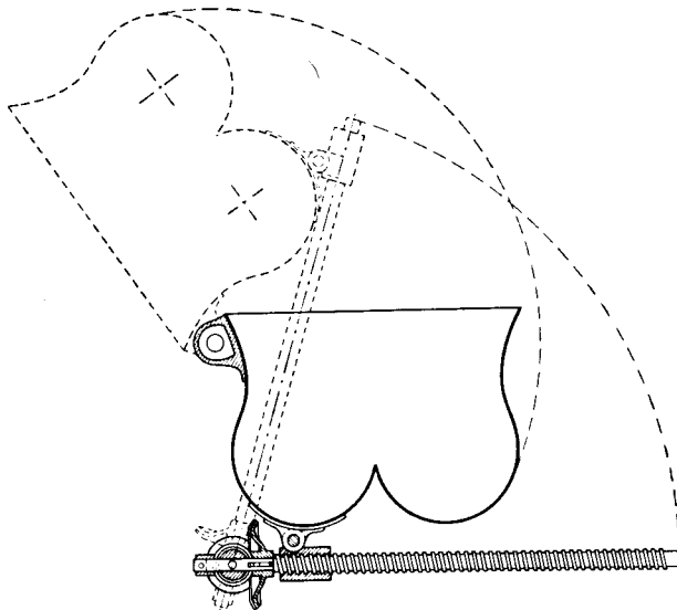
FIG. 210. Mechanism for tilting the kneader.
