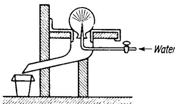
FIG. 39. Removal of mercury fulminate from the reaction flask to a rubber bucket, according to Budnikov et al. [61].
